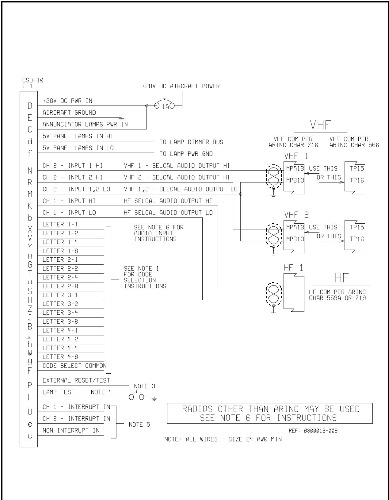
Figure 2 - CSD-10-9 and -10 Wiring Diagram
