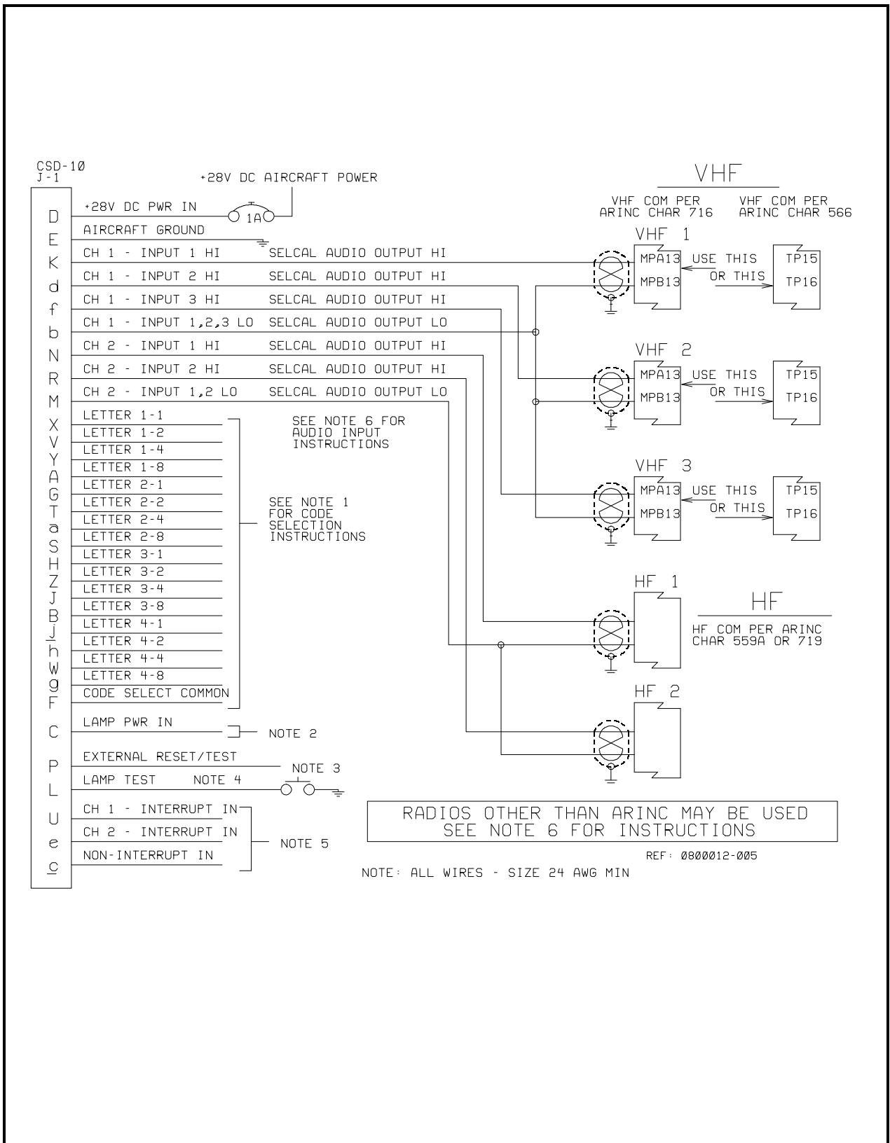
Figure 1 - CSD-10-5 thru -8 Wiring Diagram
