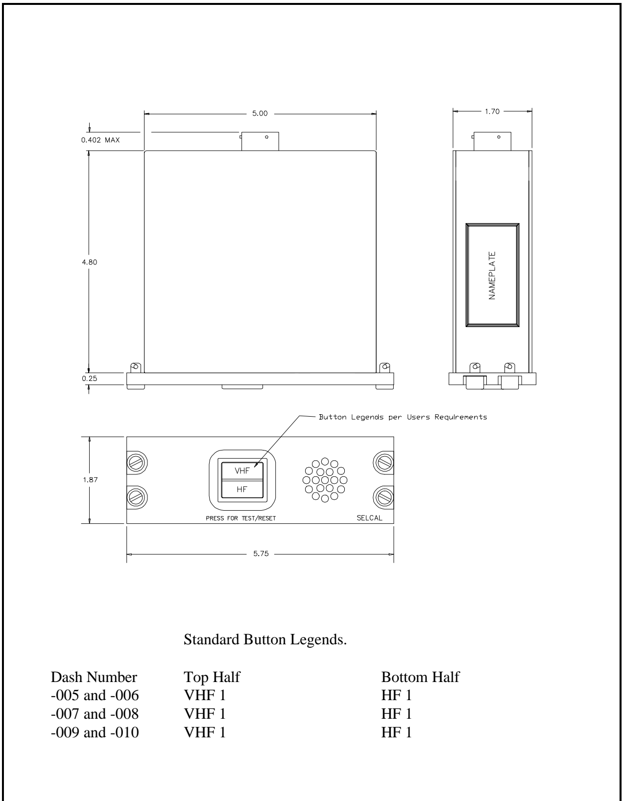
Figure 3 - Outline Drawing
