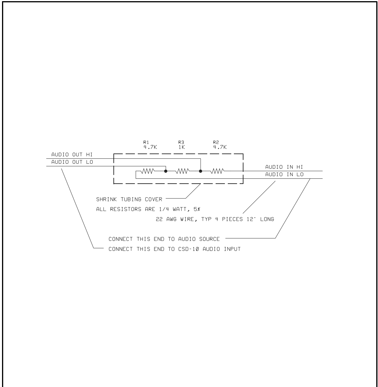
Figure 5 - 20 dB Attenuator
